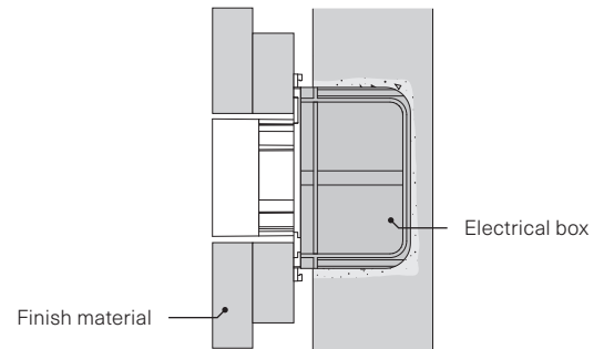
Shim up (suitable for hard material)
